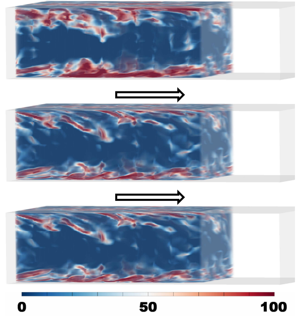
Figure 7: FTLE: As in for the local methods, we keep the color map unvaried for all three figures, but the FTLE field visualized has been computed from the original field (top), the 2nd (middle) and the 4th approximation (bottom). Observe that the focusing on the energetically most dominant scales of motion energy yields a more crispy and detailed output with finer lobes. Adding two more modes does not change the output, even though just two modes were used for the first approximation. This indicates that the dissipative scales have to be interpreted as “noise” in the context of integration-based feature extraction. We refer to the text for further discussion.
