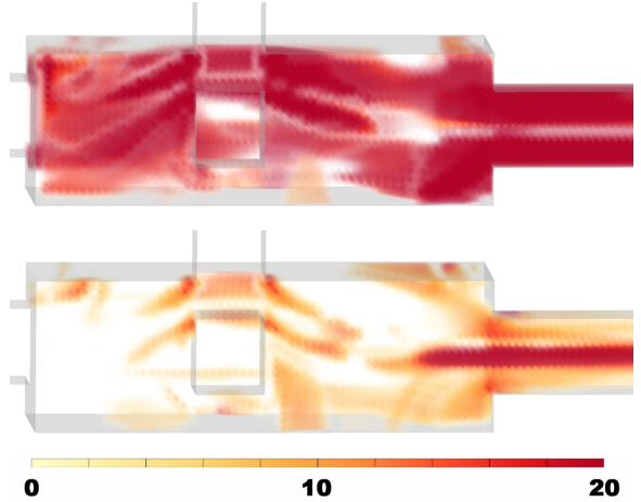
Figure 4: Vorticity method: Both figures show the same threshold, but the scalar vorticity field has been computed from the original field (top) and the 5th approximation (bottom), respectively. We see a strong reduction of the structures in the back of the top picture when taking the most dominant modes only. In the outflow, the vorticity field based on the most dominant modes reveals one instead of two vortices. This effect is called vortex braiding. For further discussion we refer to the text.
