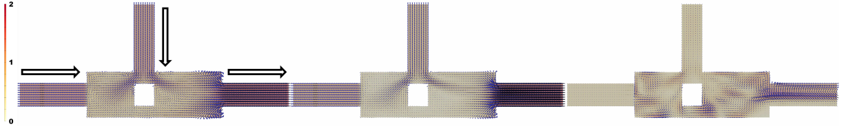
Figure 2: Flow in a T-junction and its POD modes, constructed from 100 snapshots. From left to right: the actual flow (inflow from the left and top), its first and 6 th POD mode. The background color is the norm of the point wise contribution of the respective mode to the reconstruction in the respective time step. We see that the mode with the highest energy content gives a simpler instantaneous flow pattern that the flow itself and reveals structures buried under other scales. The arrows are scaled according to norm of the respective vectors in the single modes
