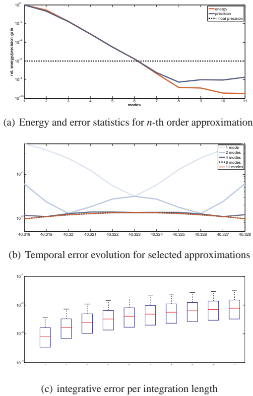
Figure 5: (a) The relative energy and precision gain of the i th order approximation compared to the (i - 1) st approximation. The precision is calculated using the time averaged relative L^2 -error of the respective approximations. (b) The function graph of the L^2 -error plotted against time for several approximations. (c) Box plot of the integrative error of the 8-th order approximation. The groups represent particles seeded at all cell centers and advected for n \cdot dt , dt being the constant time-sampling distance of the data set.
